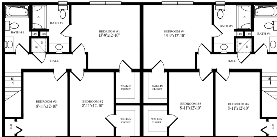
Springfield 2-Story Duplex 2nd floor
